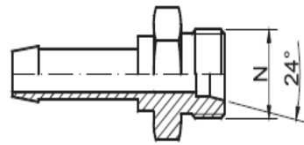
Priklučak D / Stright male fitting type "D"
