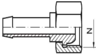
Priklučak A / Stright female fitting type "A"
